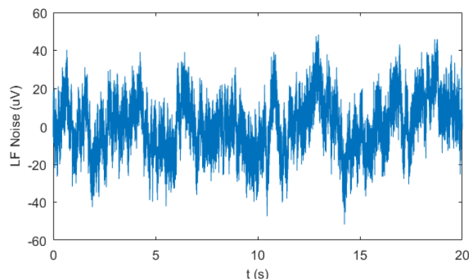
Figure 5. Low frequency output noise (0.03 Hz to 10 Hz)
