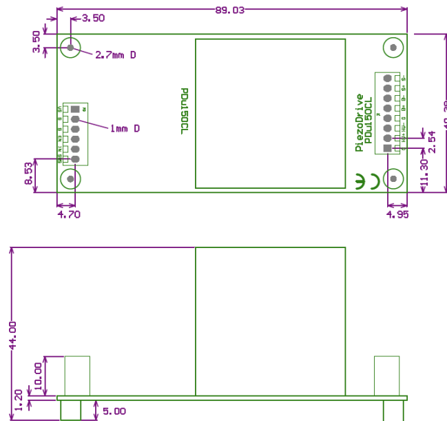
Figure 12. Dimensions (mm)
