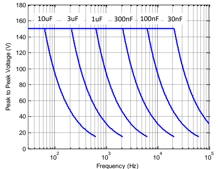
Figure 3. Power Bandwidth
