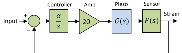
Figure 7. Feedback structure of the PDU150CL
