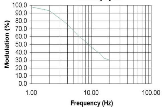
Modulation (%) Vs. Frequency (Hz) 50% duty cycle
